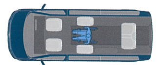
2 Row Passenger Conversion 6 Passengers and 1 Wheelchair OR 4 Passengers and 2 Wheelchairs
